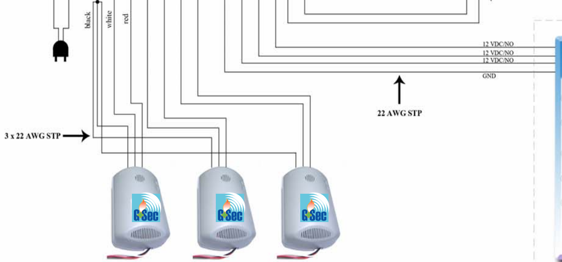
GAS DETECTOR
